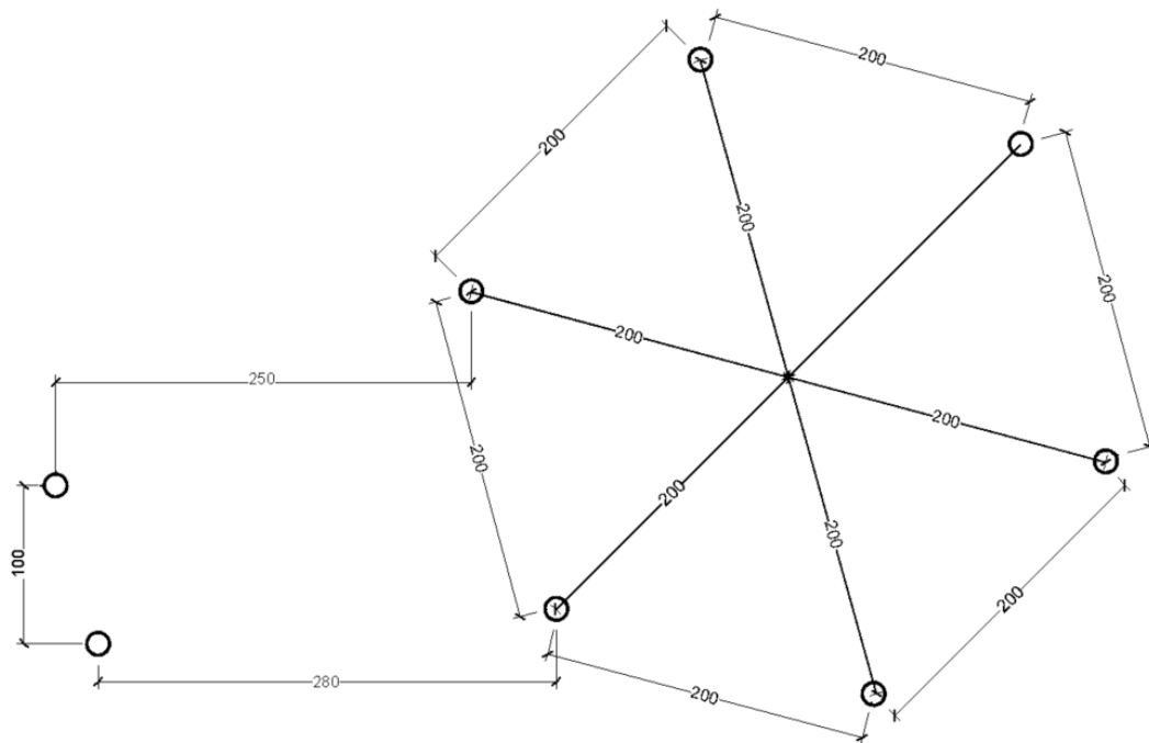
Funderingsplan
